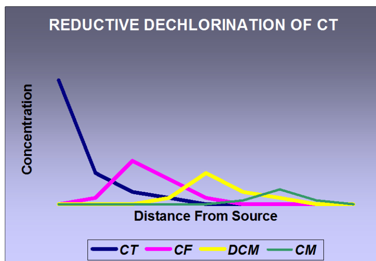
Figure 9-5. Hypothetical reduction of carbon tetrachloride with Degradation Products (carbon tetrachloride=CT [CCL 4 ], CF=chloroform [CCl 3 H], DCM=dichloromethane [CCl 2 H 2 ], CM=chloromethane [CClH 3 ])
