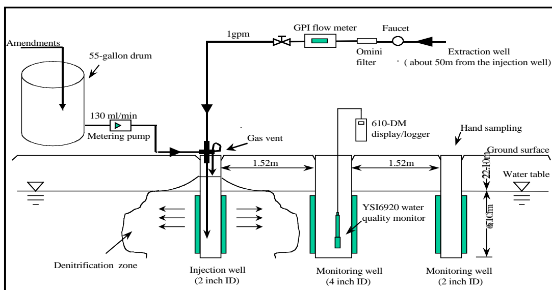
Figure 8-6. Modified schematic diagram of continuous denitrification field test
