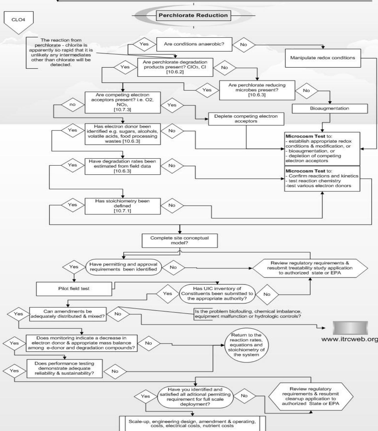
Figure 10-1 Bioremediation of Perchlorate in Ground Water
