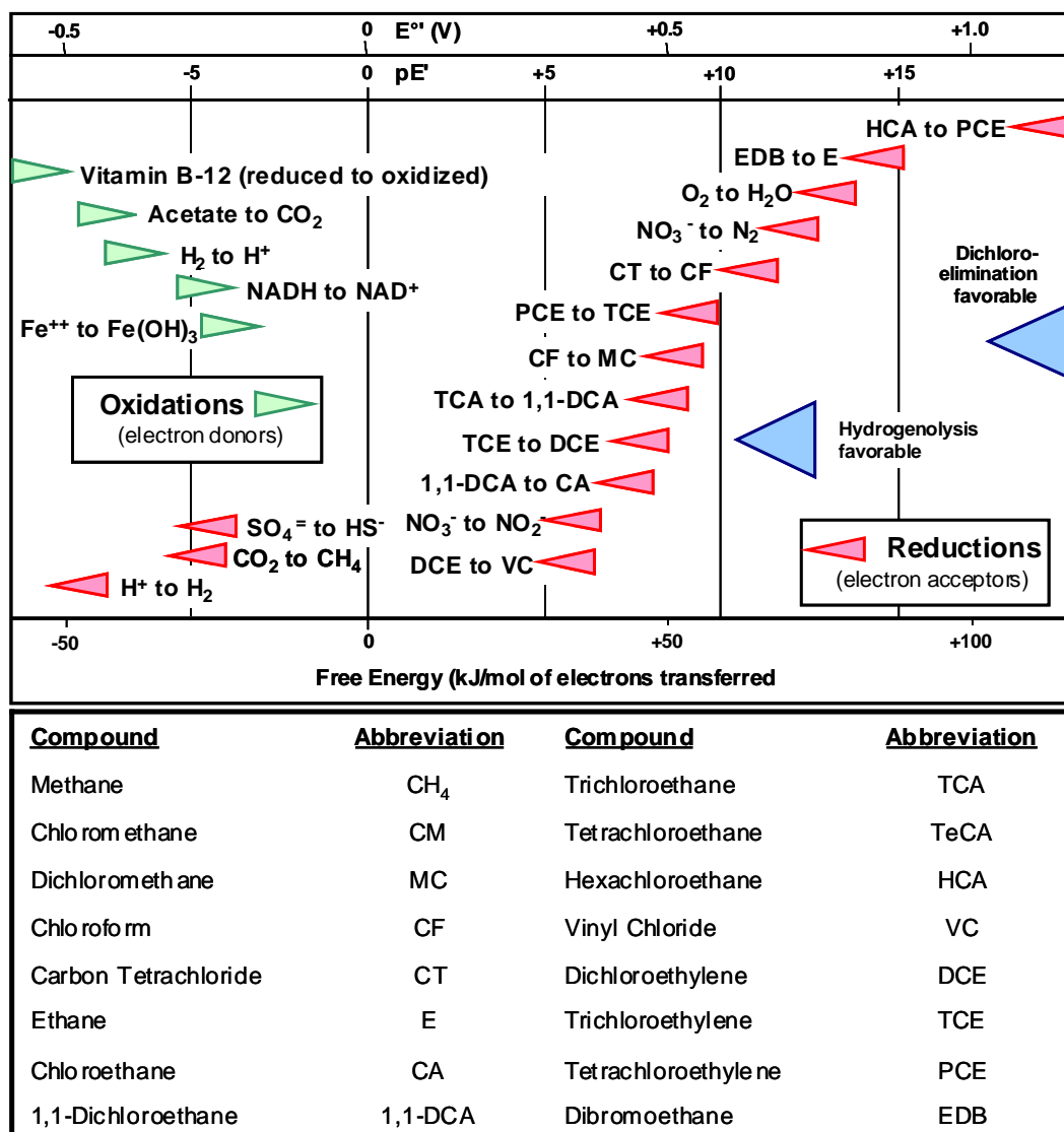
Figure 9-3. Half-reaction potentials for ORP of halogenated aliphatic compounds: potential electron acceptors and electron donors. Bases of arrows align with the potentials of the half
