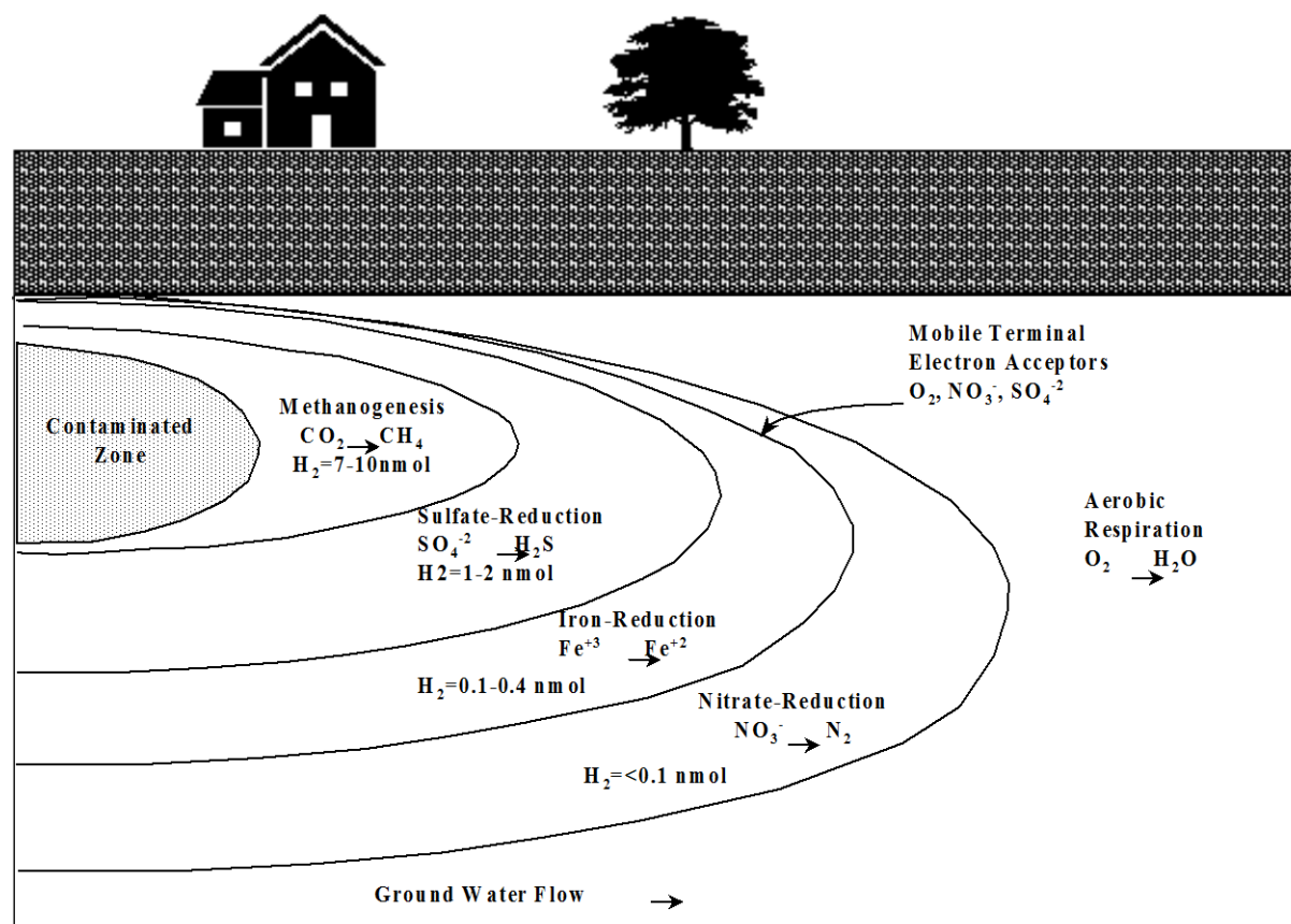
Figure 3-2 Idealized Terminal Electron Accepting Process
