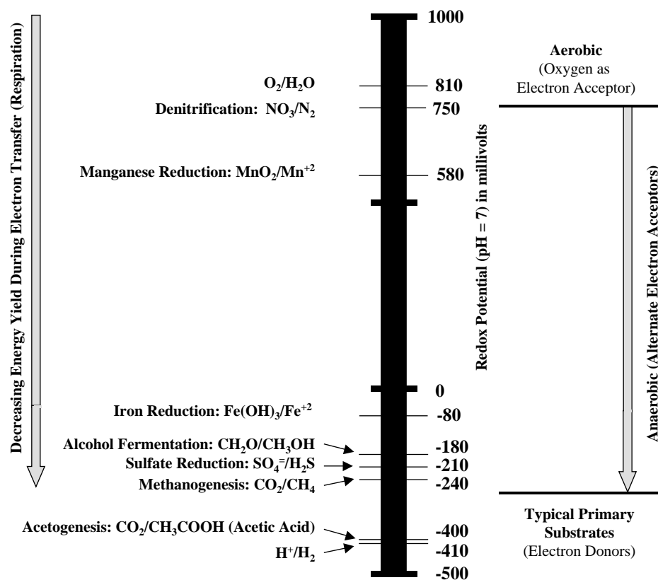
Figure 3-1 Estimated oxidation-reduction potentials of commonly monitored chemical species.
