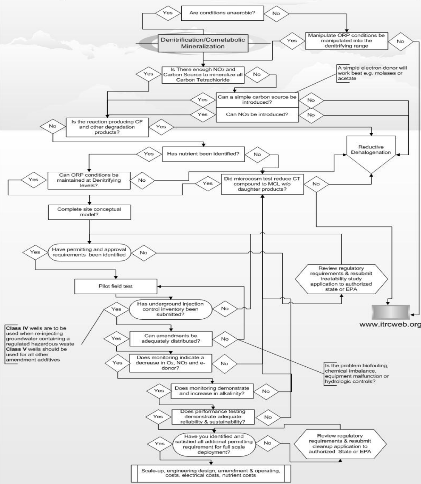
Figure 9-2 In Situ Bioremediation of Carbon Tetrachloride
