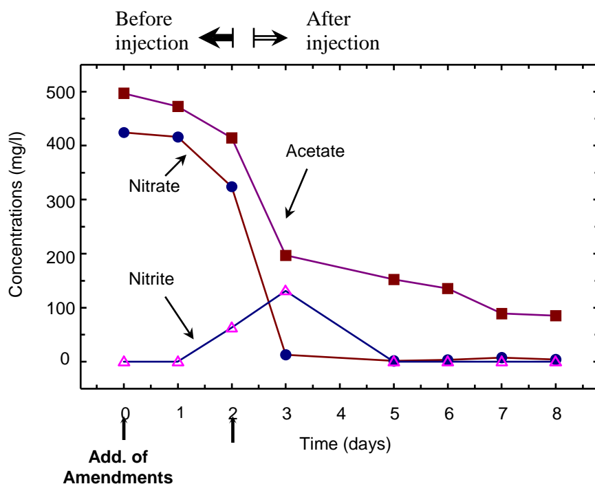
Figure 8-4. Reaction Concentration Curves Resulting from Short Term Monitoring During and After In Situ Denitrification Test
