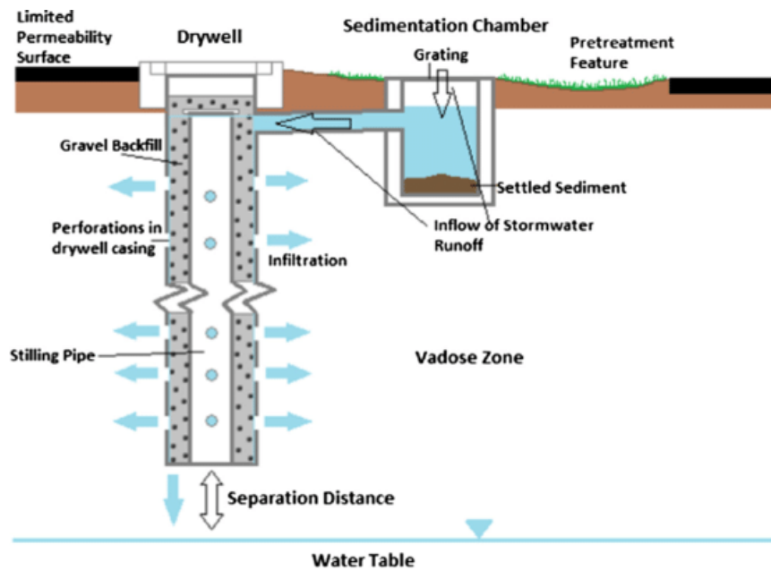
Figure 1. Dry well for stormwater management.
