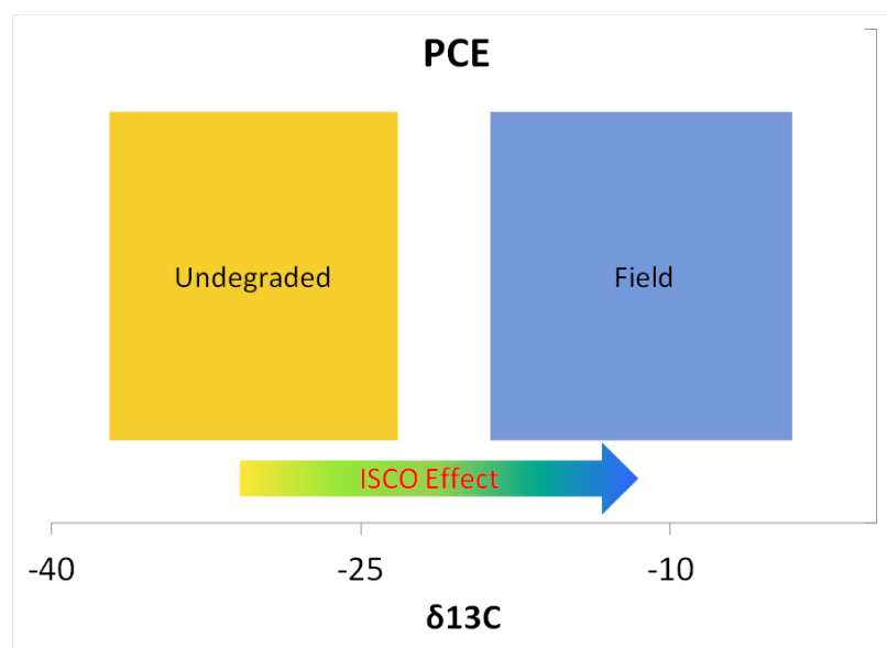
Figure 3-16. Range of degraded product and range of field measurements of \delta^{13}\text{C} of the PCE after ISCO.
