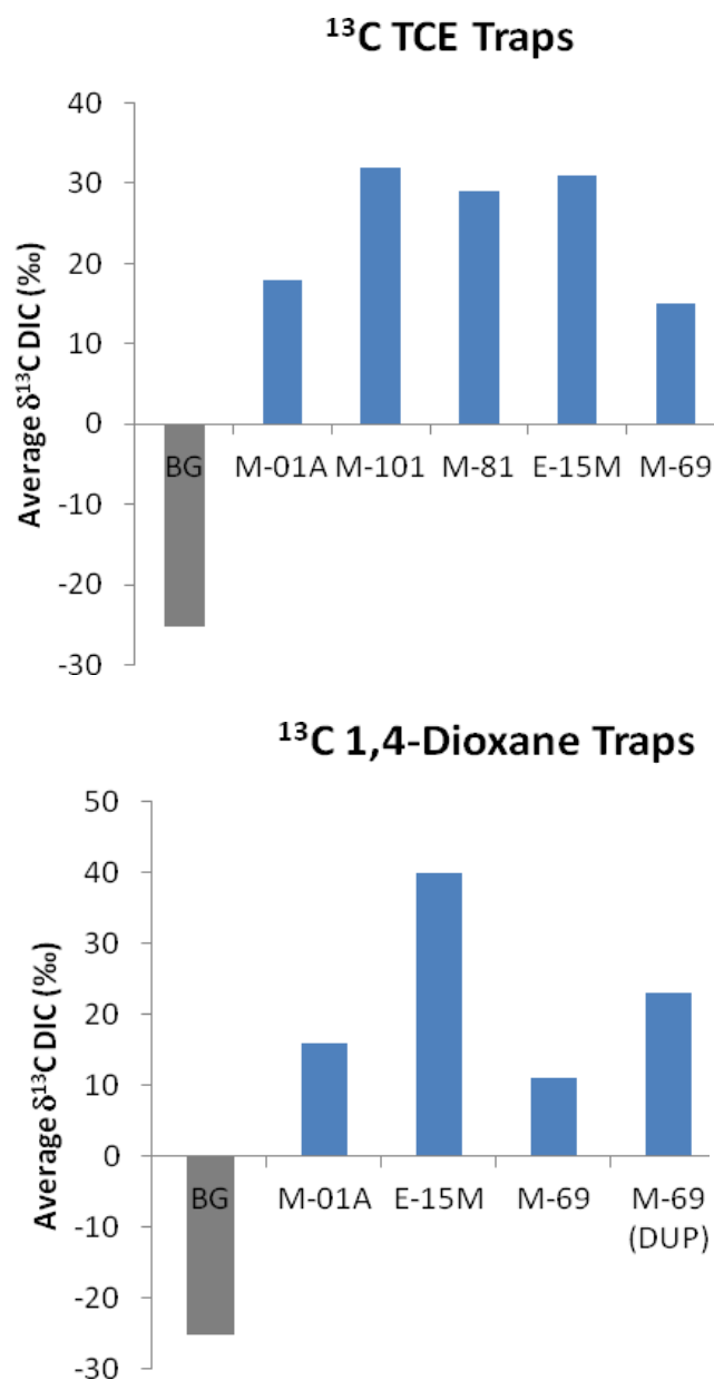
Figure A.8-4: SIP results for ^{13}\text{C} incorporation into DIC (carbon dioxide) for ^{13}\text{C} TCE and ^{13}\text{C} 1,4-dioxane baited Bio-Traps ® from select monitoring wells.
