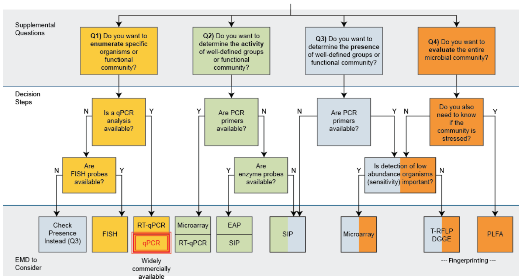
Figure 2-3. Decision tree.
