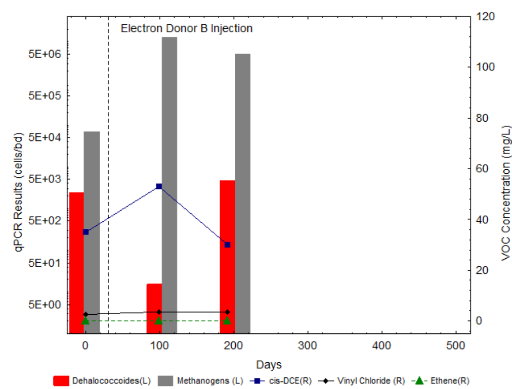
Figure A.4-2. Performance monitoring results through day 200.
