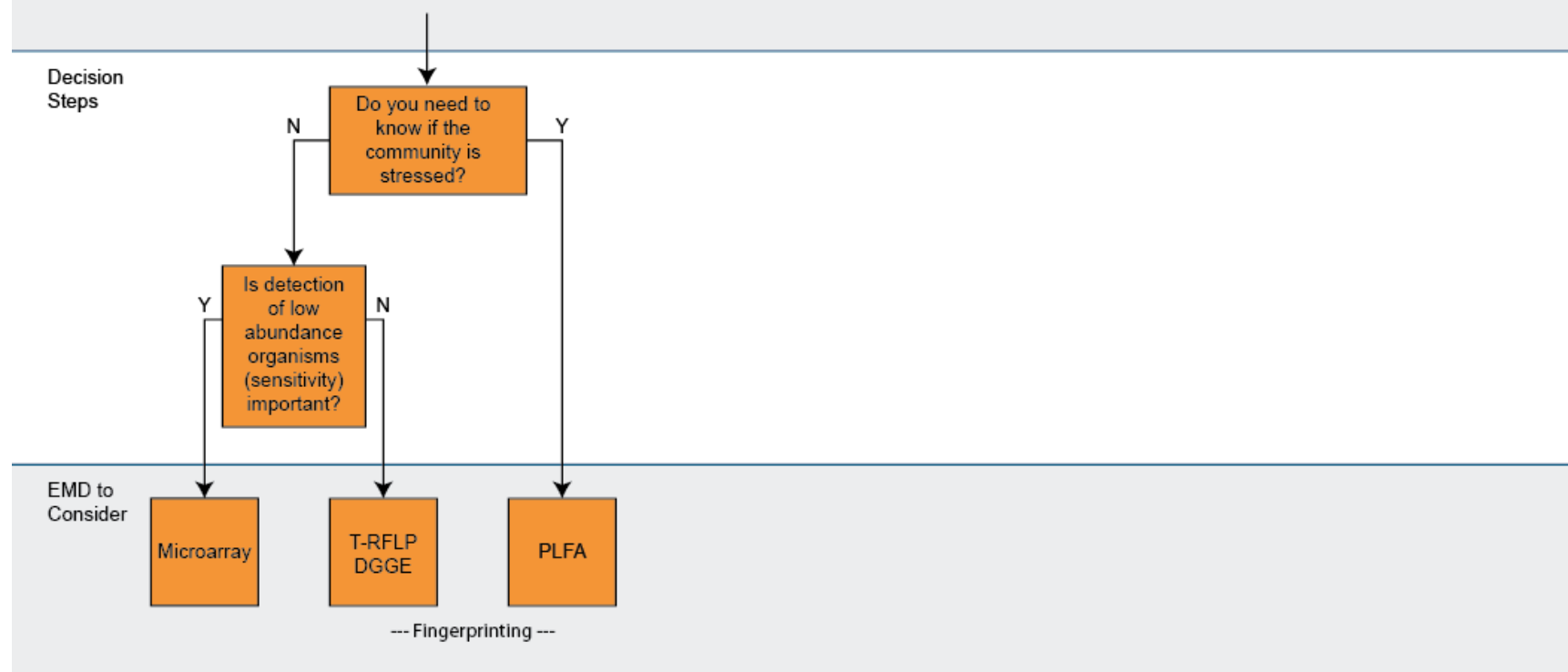
Figure 2-9. Decision tree.
